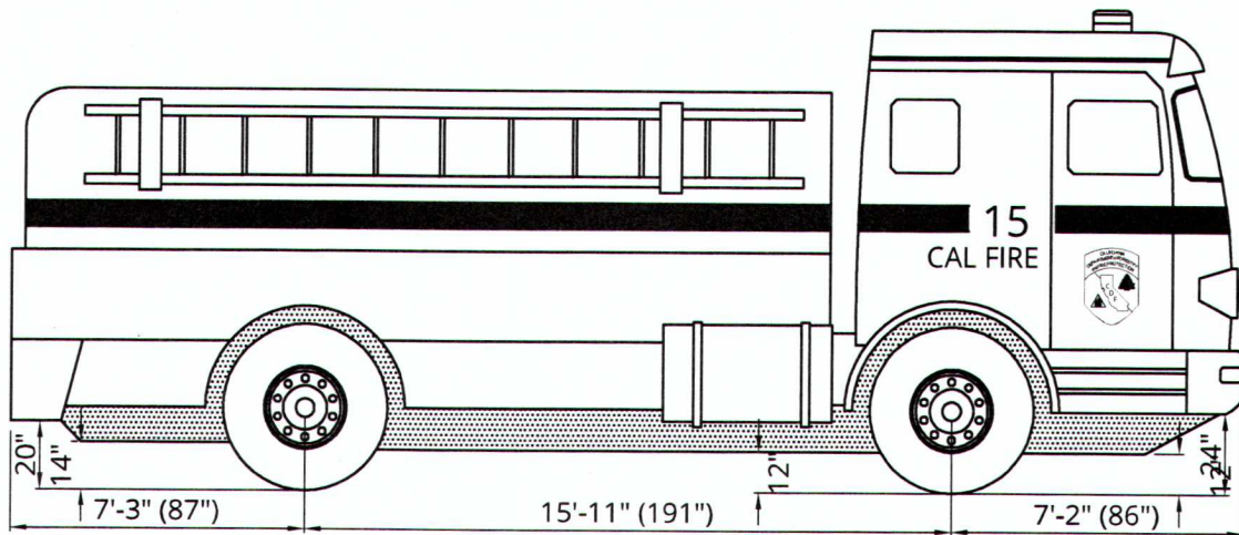
DESIGN TRUCK SCALE: 1"=5'
